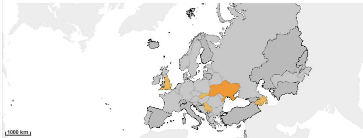
Intensity of influenza activity (EU layout map), 2020-W48
